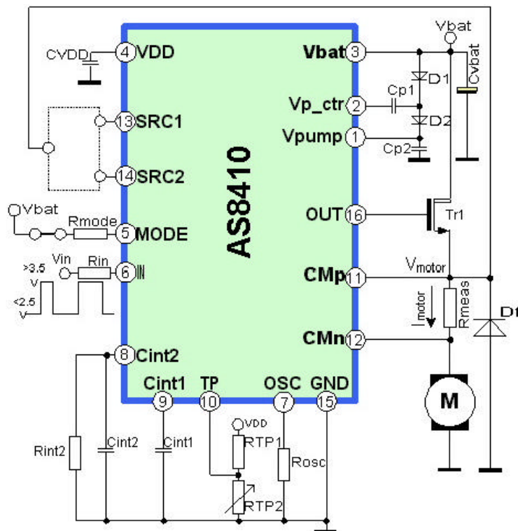
Fig. 3.1 Operating mode 1 (OM1) of the motor regulator (e.g. automotive application)
