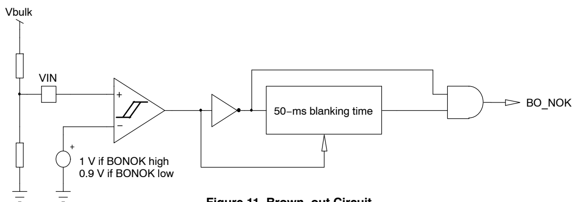
Figure 11. Brown-out Circuit
