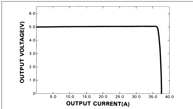
■ OVERCURRENT CHARACTERISTICS (P150E-5)
