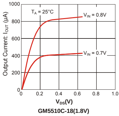
N-ch Driver Output current vs. V_{DS}
