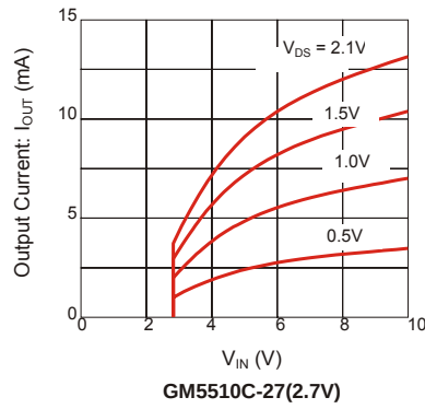
P-ch DRIVER OUTPUT CURRENT VS. INPUT VOLTAGE
