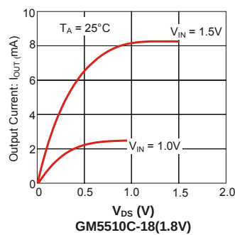
N-ch Driver Output current vs. V_{DS}
