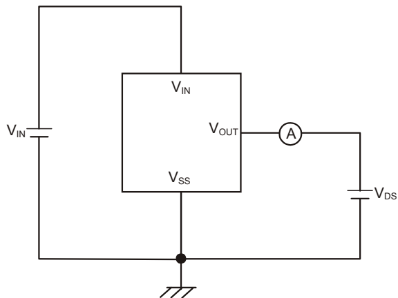
Test Circuit 3
