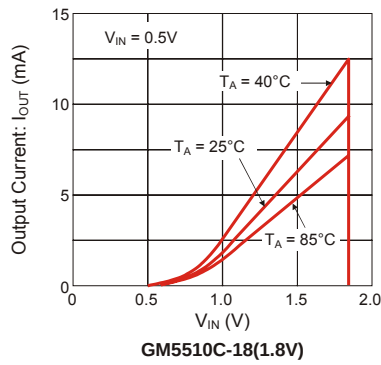
P-ch DRIVER OUTPUT CURRENT VS. INPUT VOLTAGE
