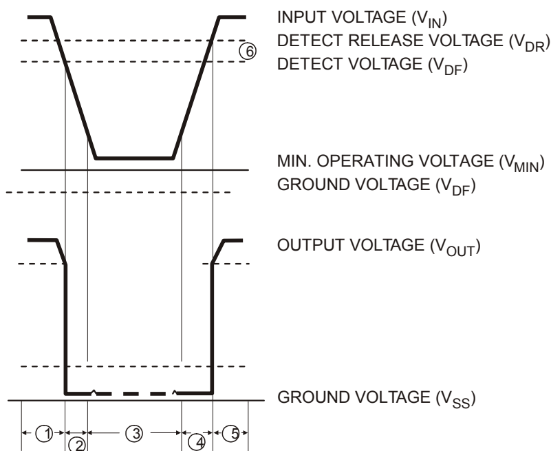
Timing Chart
