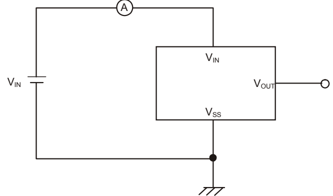
Test Circuit 2
