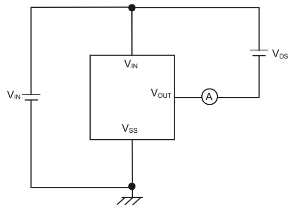
Test Circuit 4
