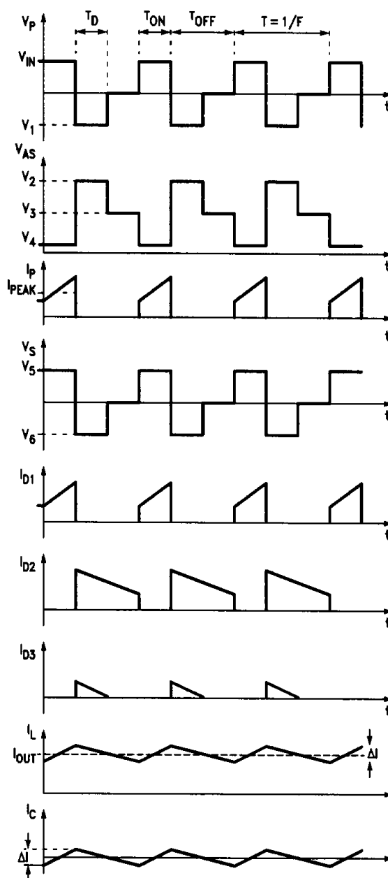
FIGURE 4. Typical Forward Waveforms
