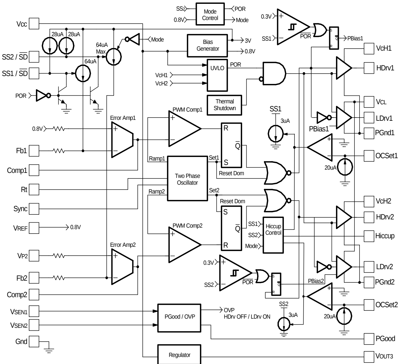
Figure 3 - IR3621Block Diagram
