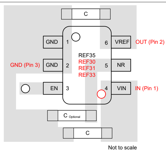
Figure 12-2. Pin Compatibility with REF30xx, REF31xx and REF33xx
