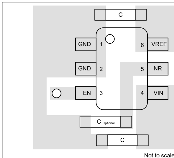
Figure 12-1. Layout Example
