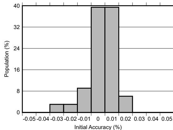
Figure 7-4. Initial Accuracy Distribution
