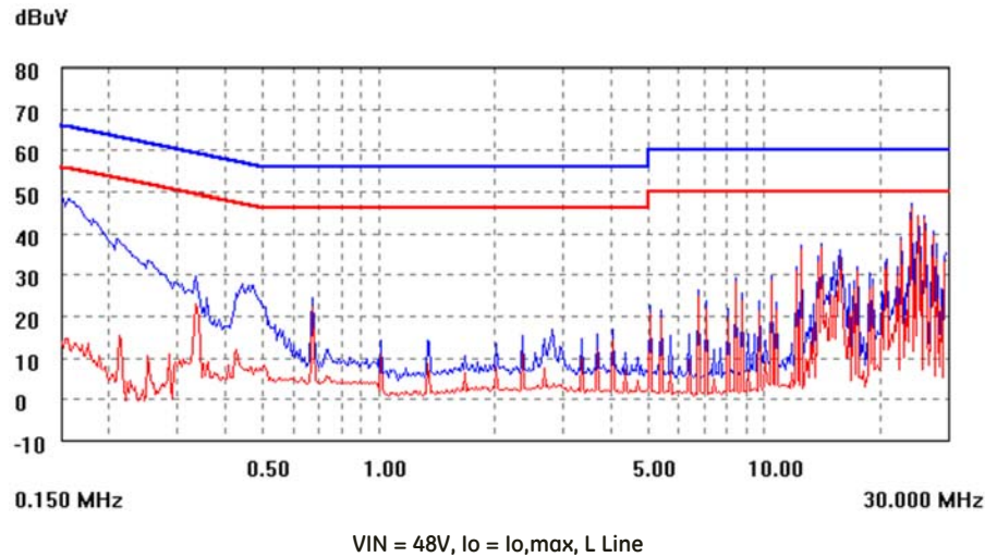
Figure 25. EMC Considerations
