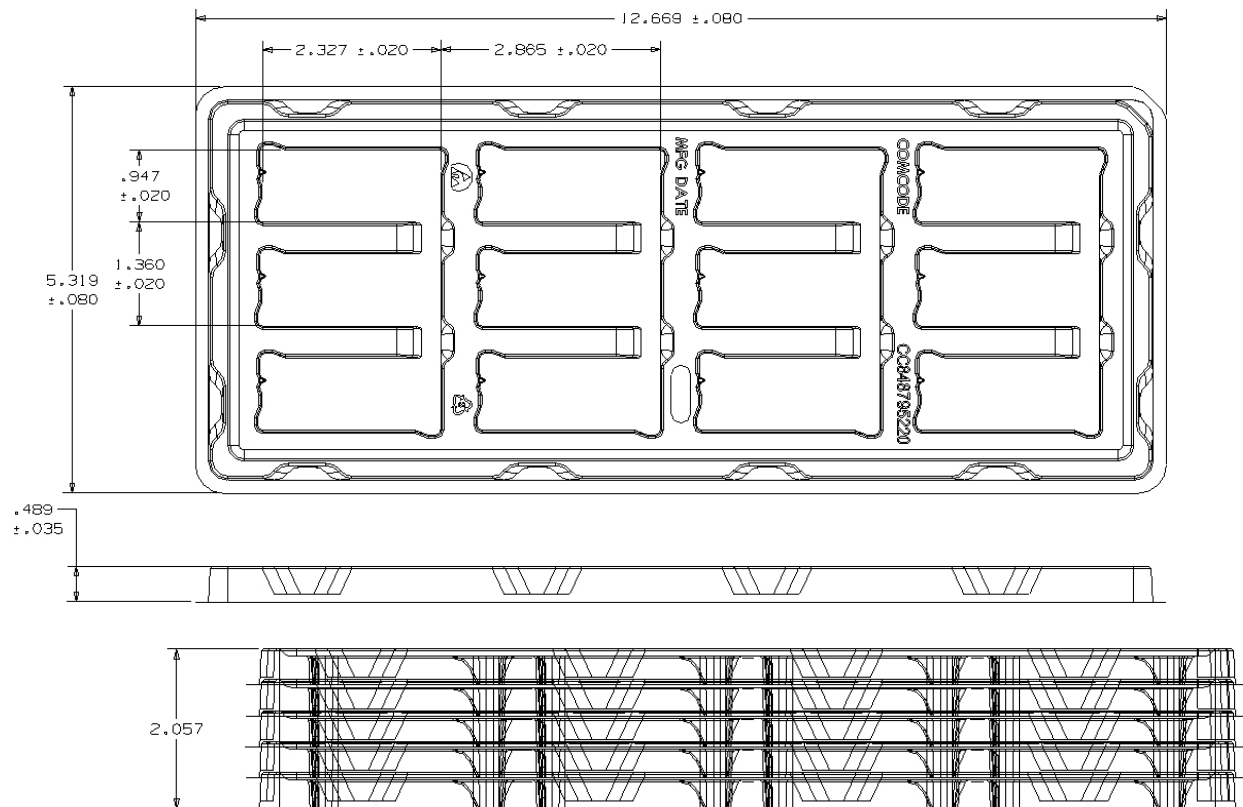
Figure 26. Surface Mount Packaging Tray
