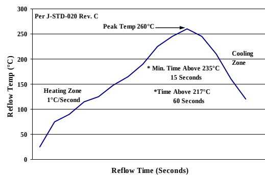
Figure 24. Recommended linear reflow profile using Sn/Ag/Cu solder.
