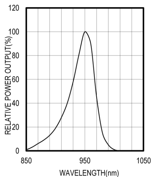
SPECTRAL OUTPUT
