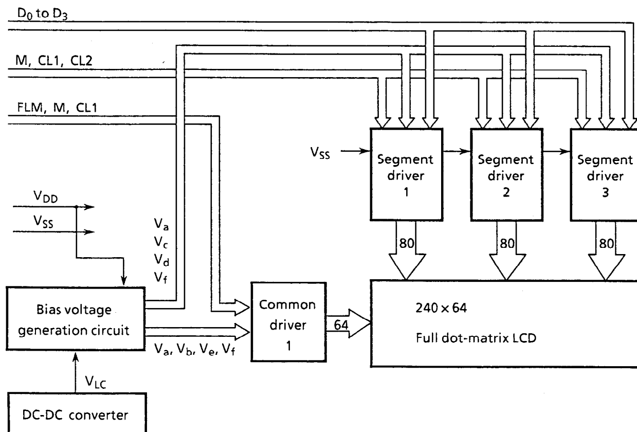
Figure 3 Block diagram
