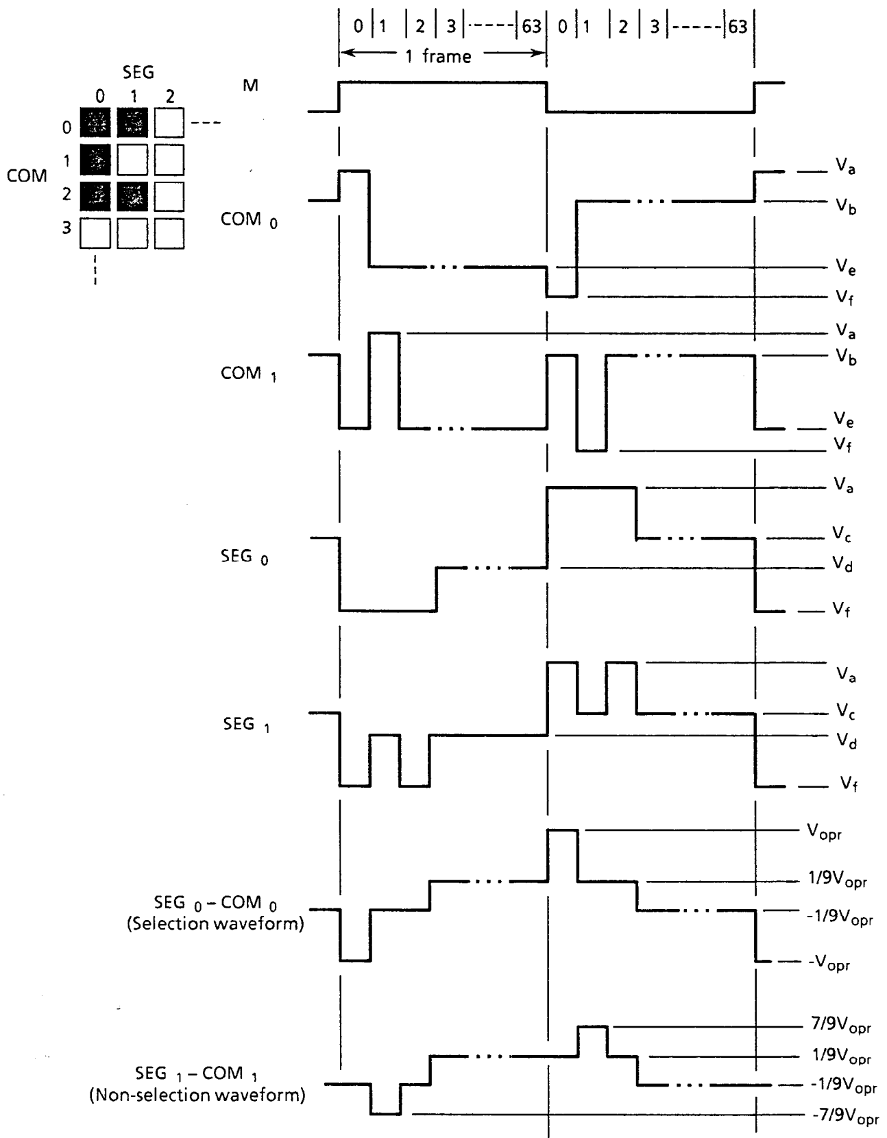
Figure 2 Drive waveform
