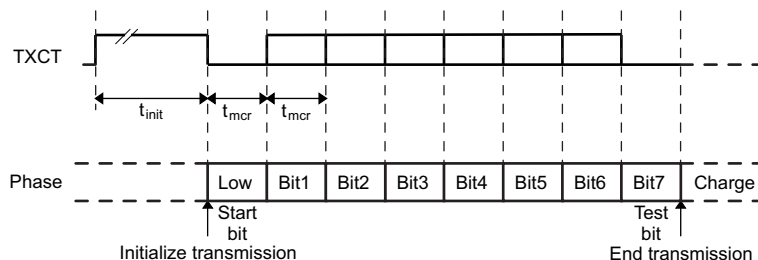
Figure 5-4. Mode Control Write Protocol (NRZ Coding)
