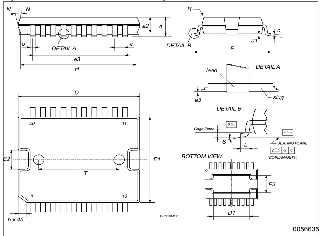
Figure 16. PowerSO20 mechanical drawing
