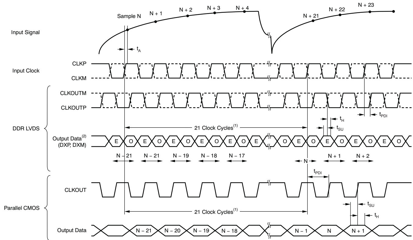
Figure 5. Latency Diagram
