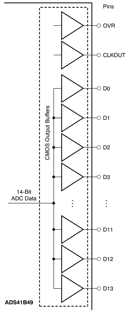
Figure 72. CMOS Output Interface
