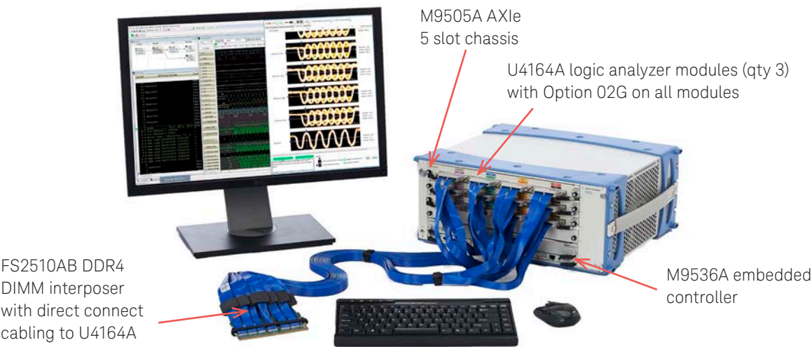
Figure 14. Typical configuration for DDR4 DIMM debug and validation for data rates greater 2500 Mb/s.
