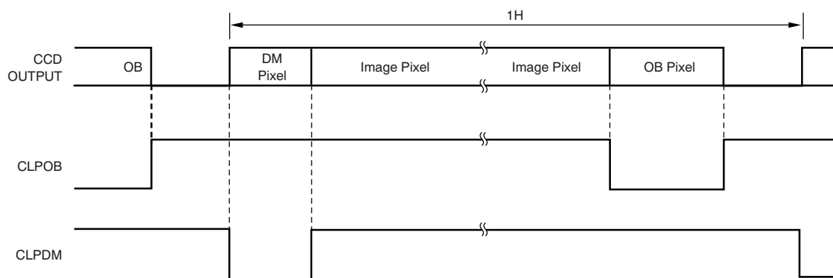
Figure 8. Timing for CLPOB and CLPDM
