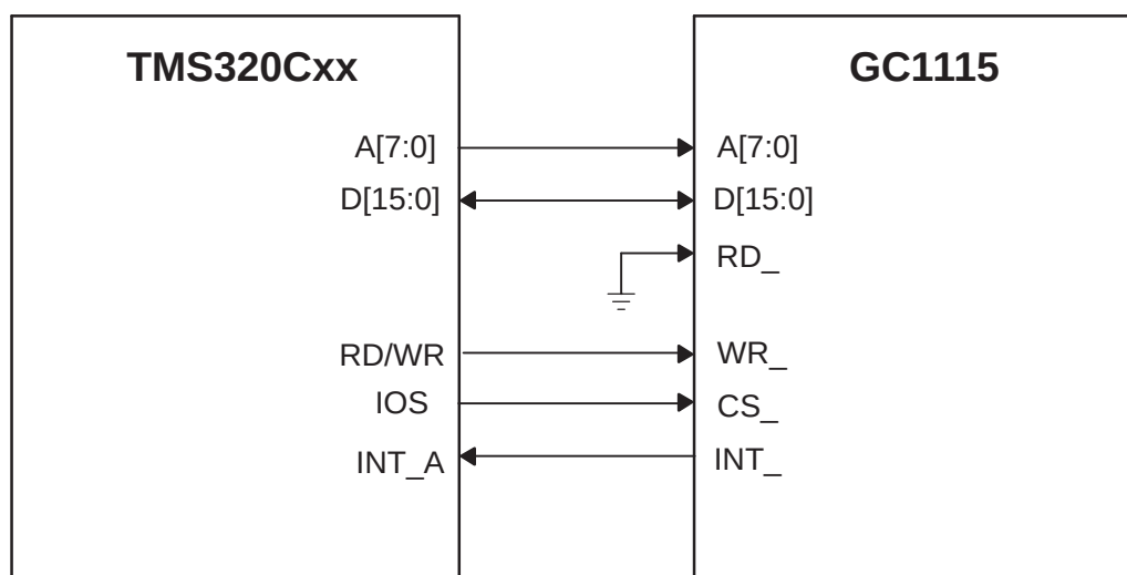
Figure 8. TMS320Cxx – GC1115 Interface
