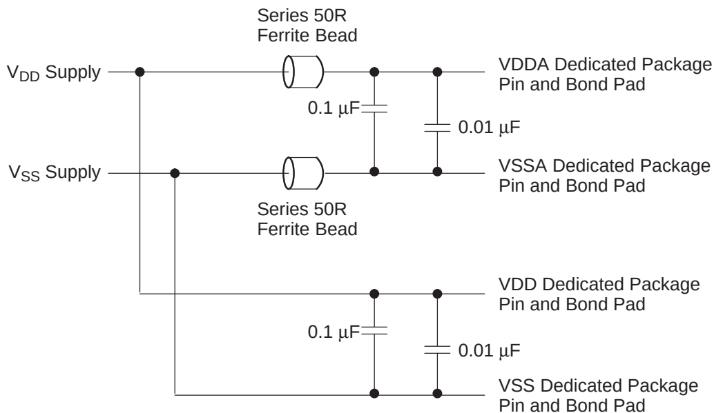
Figure 16. Power-Supply Filter
