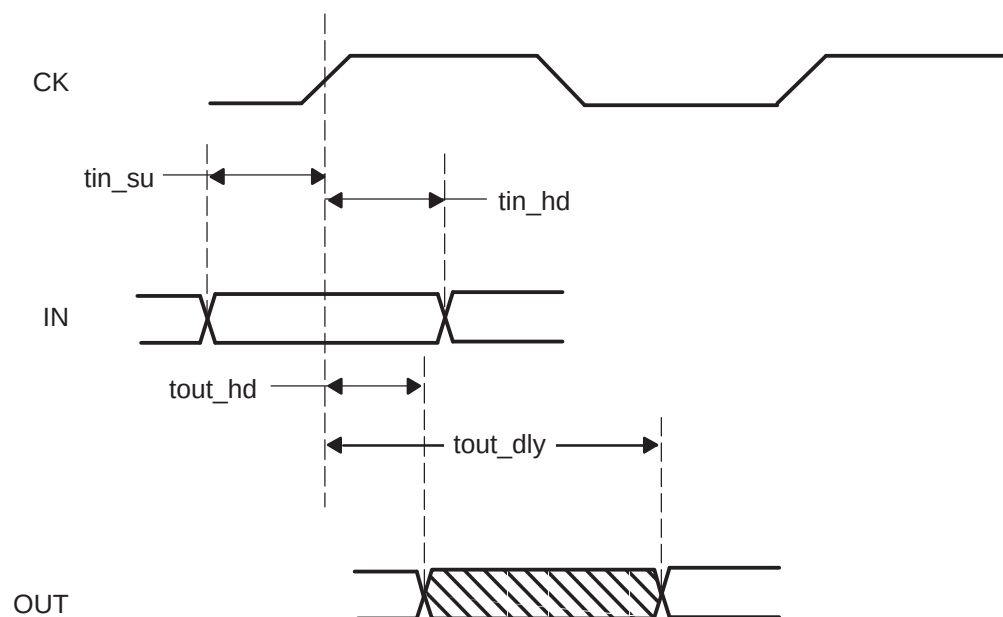
Figure 15. Generic Data Setup and Hold. Data Output Hold and Delay
