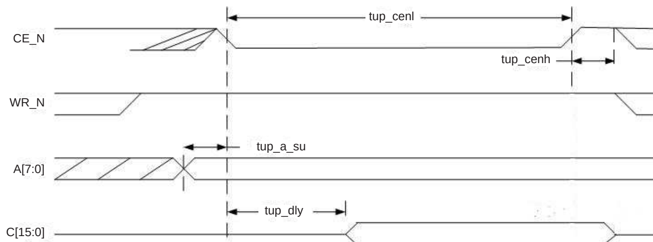
Figure 13. Read Cycle \overline{RD} Held Low
