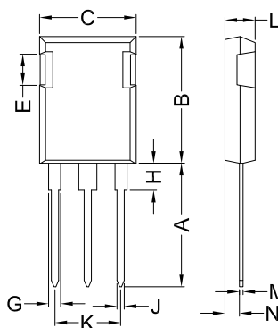
Dimensions TO-247P
