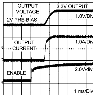
Pre-Biased Startup
