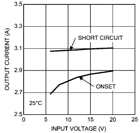
Current Limit 3.3V_{OUT} @ 25^{\circ}C
