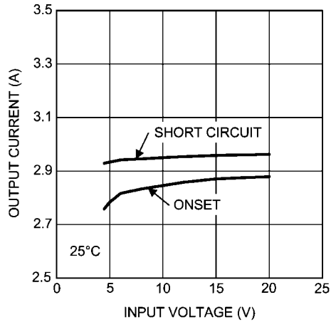
Current Limit 1.8V_{OUT} @ 25^{\circ}C
