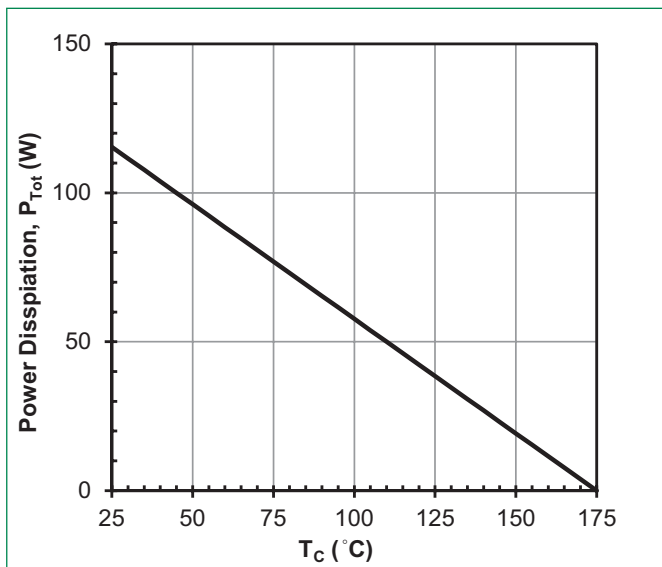
Figure 3: Power Dissipation
