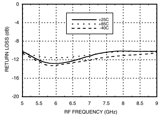
RF Return Loss vs. Temperature
