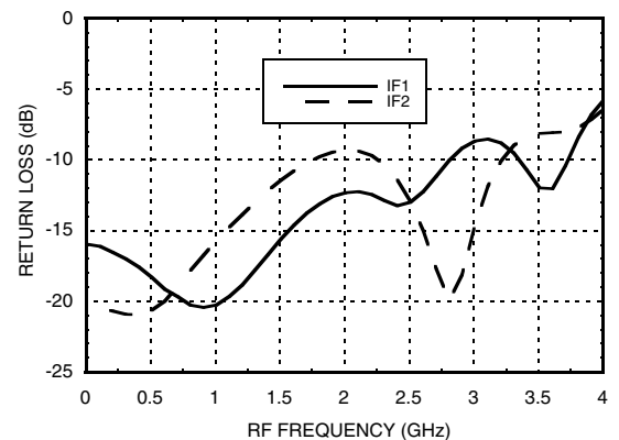
IF Return Loss [1]
