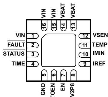
ISL9205 (16 LD QFN) TOP VIEW
