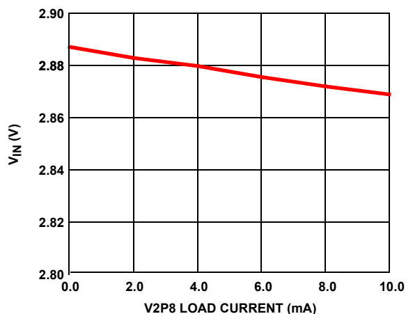
FIGURE 10. V2P8 OUTPUT vs ITS LOAD CURRENT
