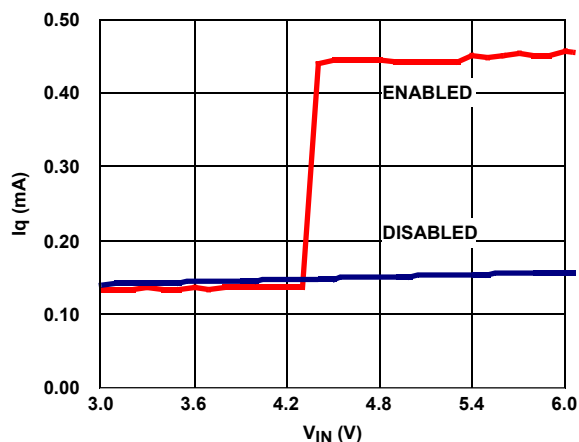
FIGURE 13. INPUT QUIESCENT CURRENT vs INPUT VOLTAGE
