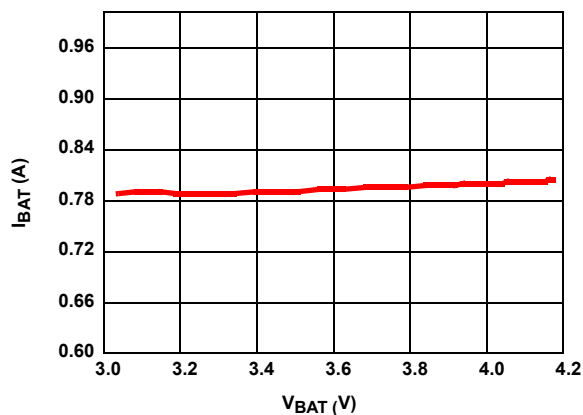
FIGURE 6. CHARGE CURRENT vs OUTPUT VOLTAGE
