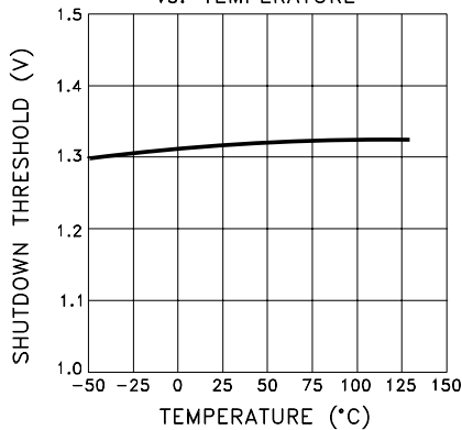
SHUTDOWN VOLTAGE THRESHOLD vs. TEMPERATURE
