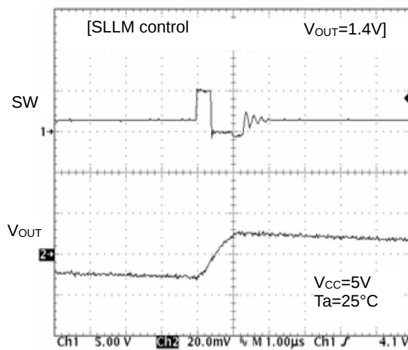
Figure 66. SW Waveform ( I_o=10\text{mA} )
