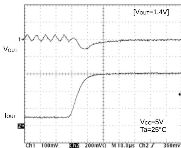
Figure 68. Transient Response ( I_O=100mA to 600mA , 10\mu s )
