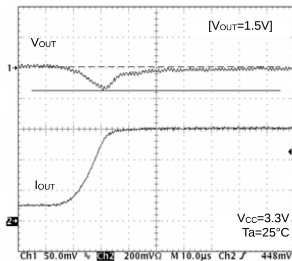
Figure 83. Transient Response ( I_o=100\text{mA} to 600\text{mA} , 10\mu\text{s} )
