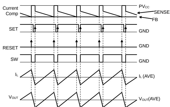
Figure 85. Diagram of Current Mode PWM Control
