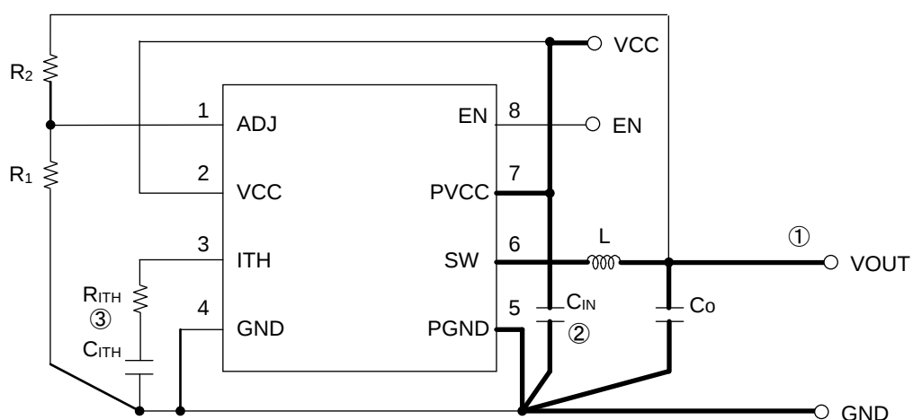
Figure 104. Layout Diagram
