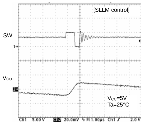
Figure 51. SW Waveform ( I_o=10\text{mA} )
