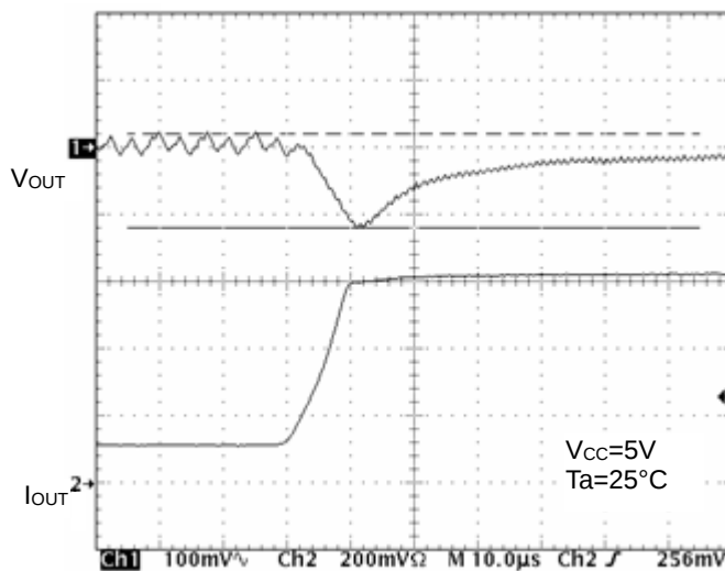
Figure 53. Transient Response ( I_o=100\text{mA} to 600\text{mA} , 10\mu\text{s} )
