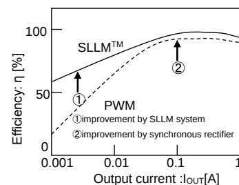
Figure 91. Efficiency
