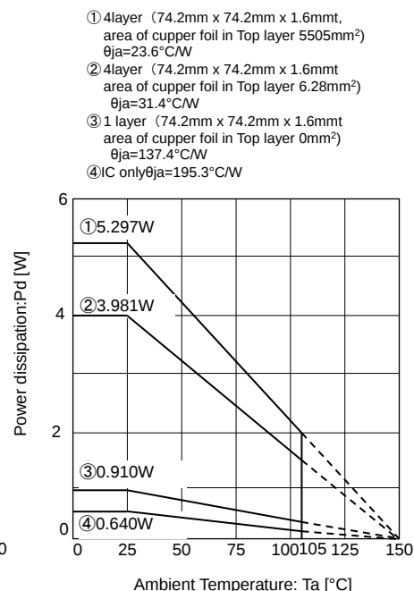
Figure 95. Thermal Derating Curve (SON008V5060)
