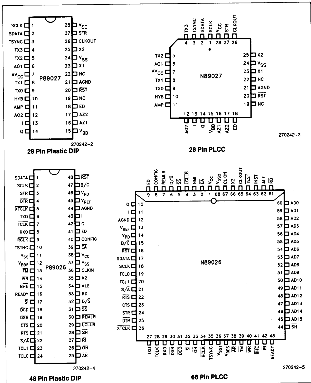
Figure 2. Device Packages
