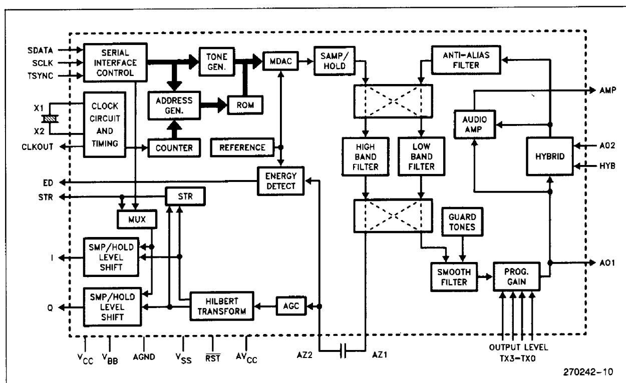
Figure 7. 89027 Block Diagram
