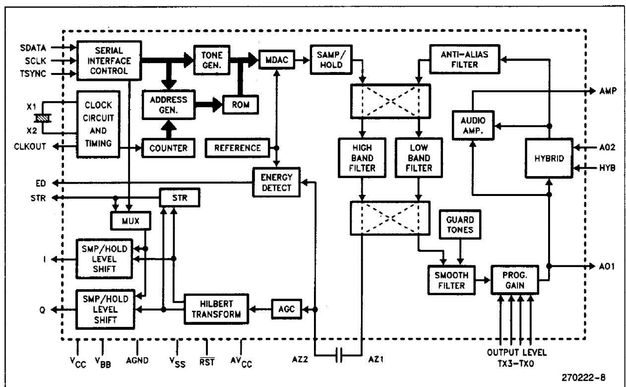
Figure 3. 89027 Block Diagram
