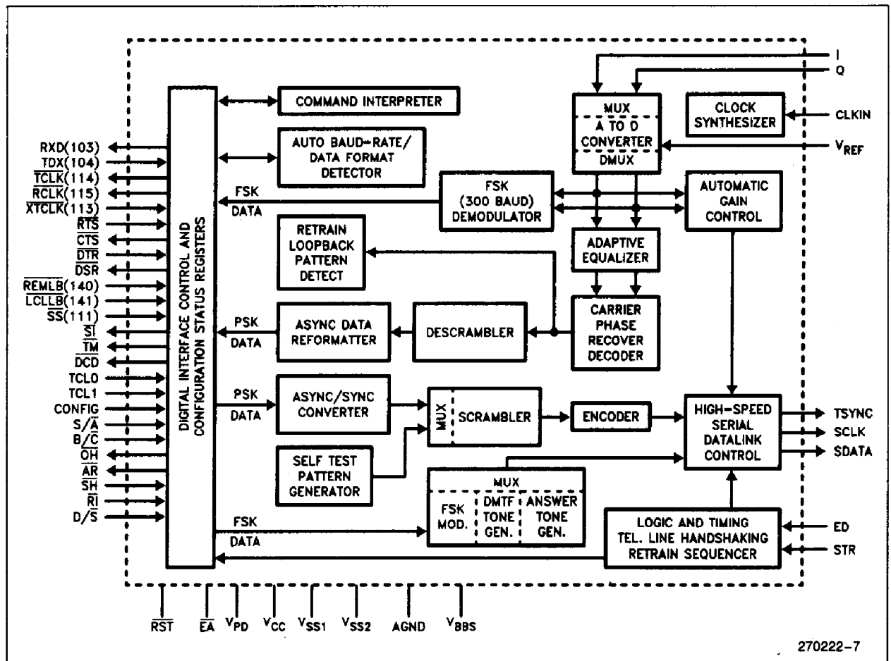
Figure 2. 89026 Block Diagram
