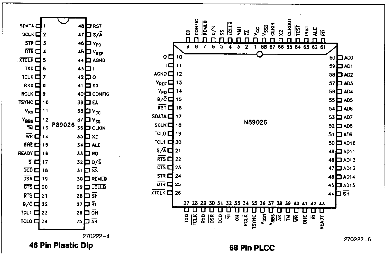
Figure 6b. 89026 Packages
