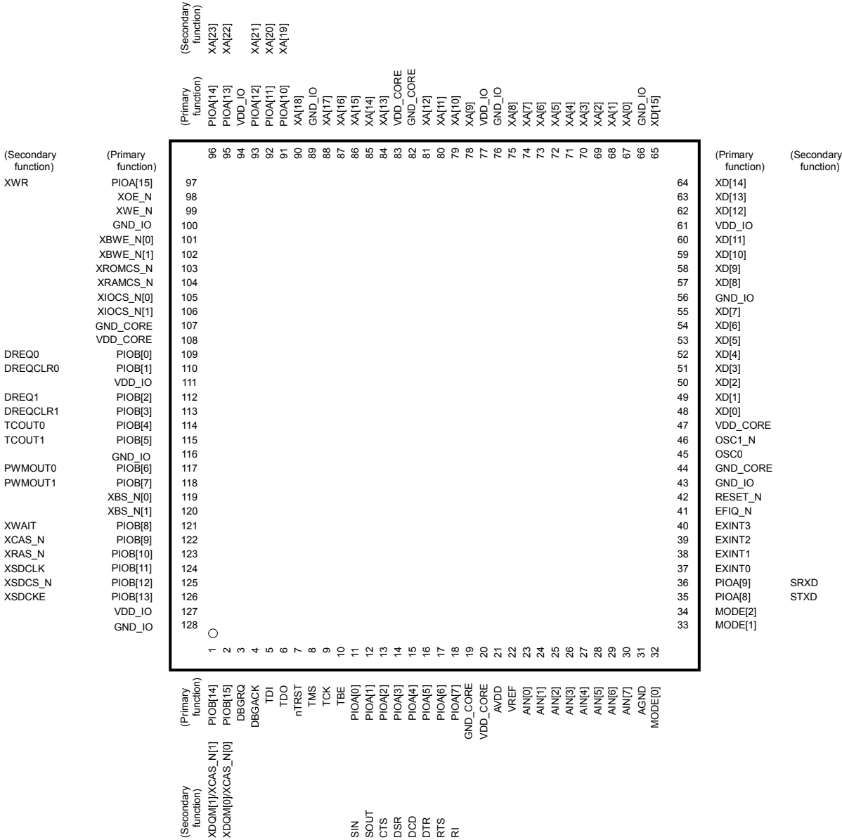
128-Pin Plastic TQFP
