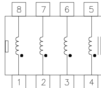
4 Line 8-Pin Schematic
