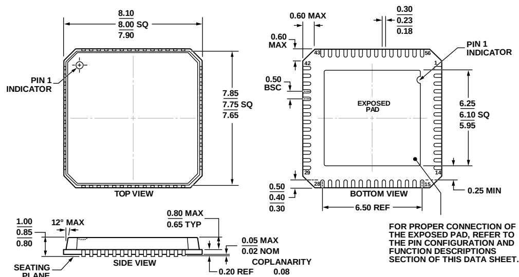
Figure 61. 56-Lead Lead Frame Chip Scale Package [LFCS_P_VQ] 8 x 8 mm Body, Very Thin Quad (CP-56-1)
