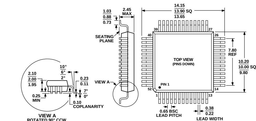
Figure 60. 52-Lead Metric Quad Flat Package [MQFP] (S-52-2)
