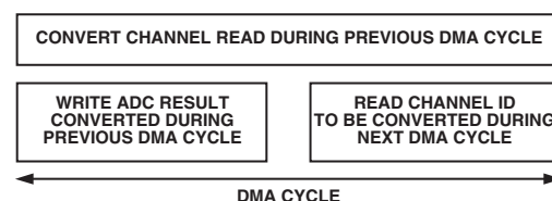
Figure 13. DMA Cycle
