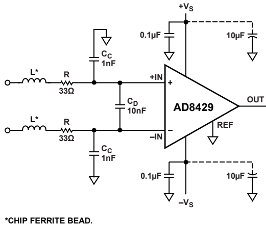
Figure 53. RFI Suppression
