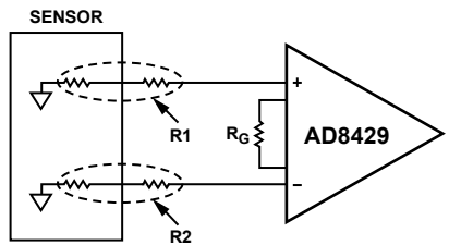
Figure 54. Source Resistance from Sensor and Protection Resistors
