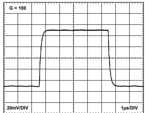
Figure 37. Small Signal Response ( G = 100 ), R_L = 10 kΩ, C_L = 100 pF
