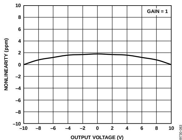
Figure 24. Gain Nonlinearity ( G = 1 ), R_L = 10\text{ k}\Omega
