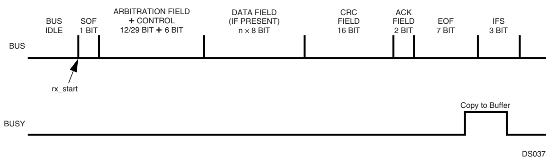
Figure 31. Receive Timing
