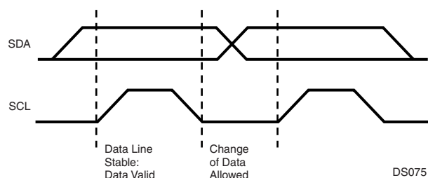
Figure 69. Bit Transfer
