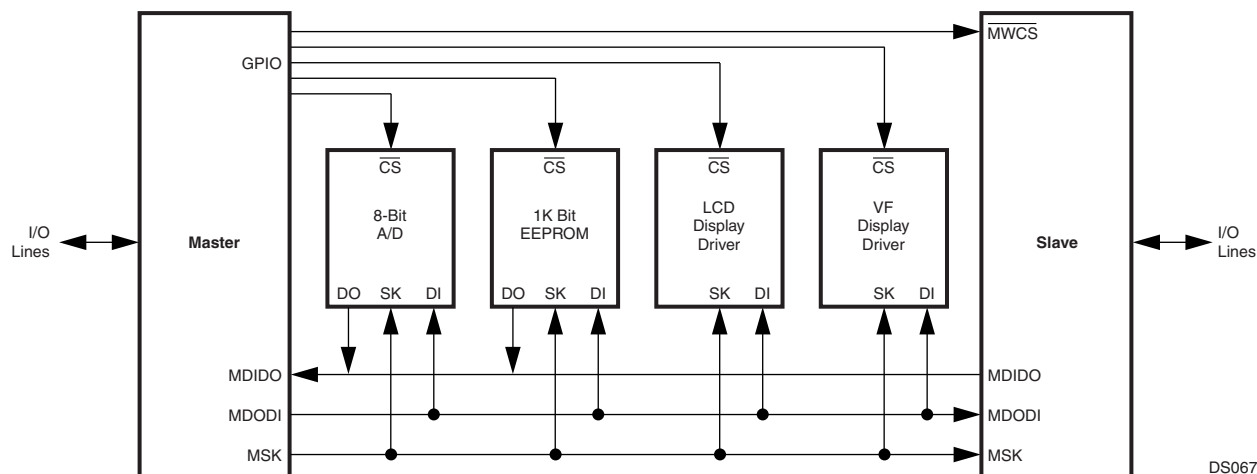
Figure 61. Microwire Interface
