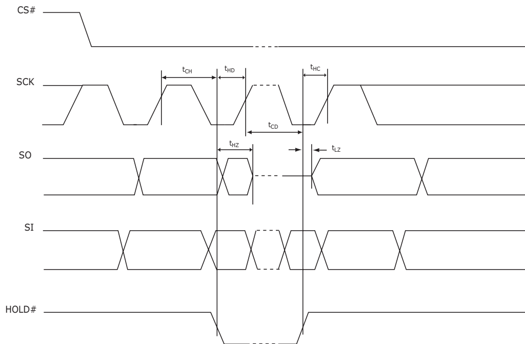
Figure 21. HOLD# Timing
