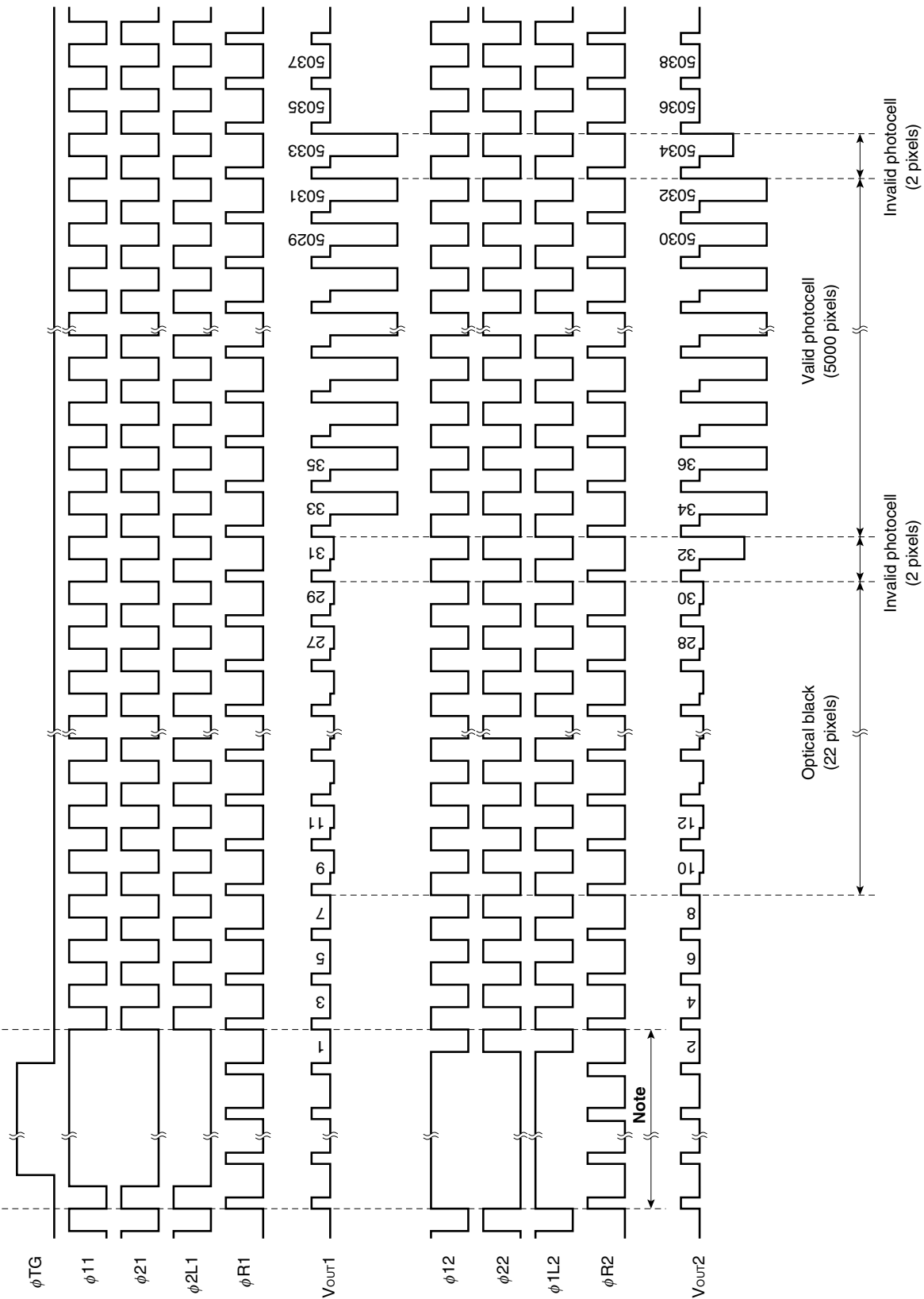
TIMING CHART 4 (In phase operation)
