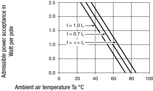
Fuses 6.3 x 32 mm (2-pole, per pole)
