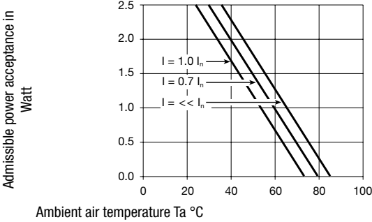
Fuses 5 x 20 mm (1-pole)
