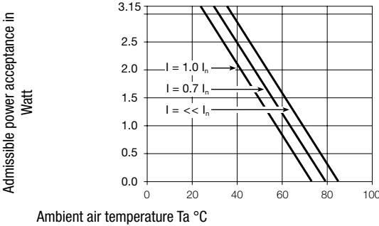
Fuses 6.3 x 32 mm (1-pole)
