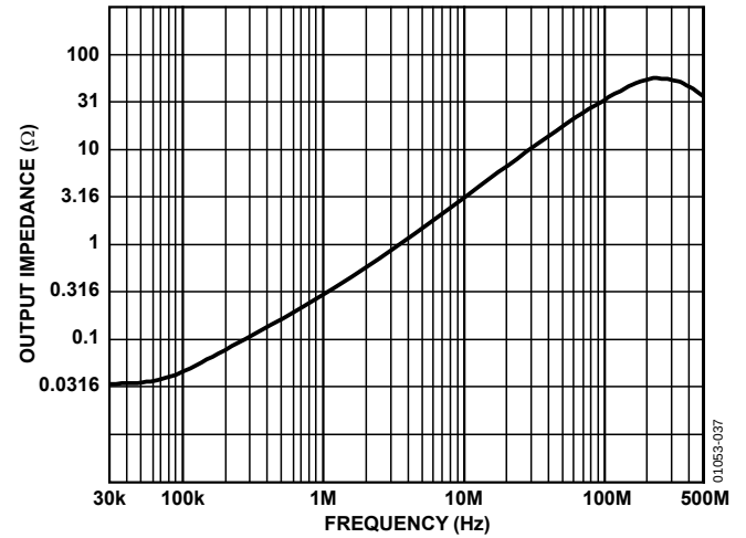
Figure 37. Output Impedance vs. Frequency, V_S = \pm 12\text{ V}
