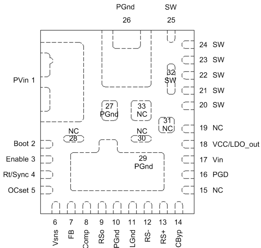
PIN DIAGRAM 5mm X 6mm POWER QFN Top View
