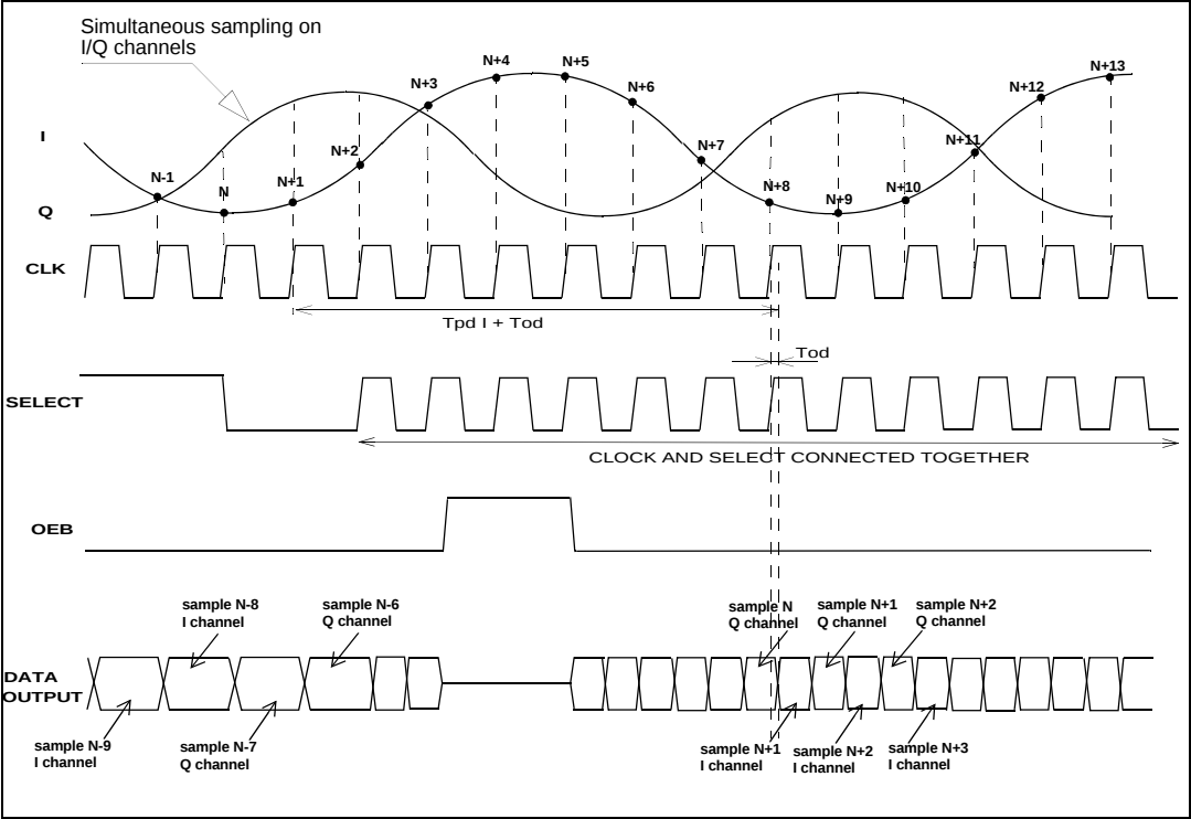
Figure 2. Timing diagram
