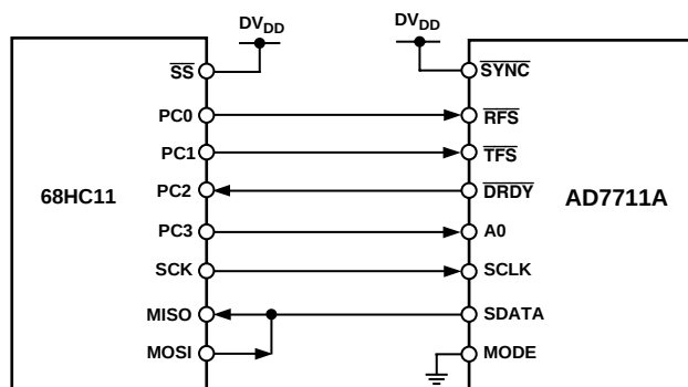
Figure 18. AD7711A to 68HC11 Interface
