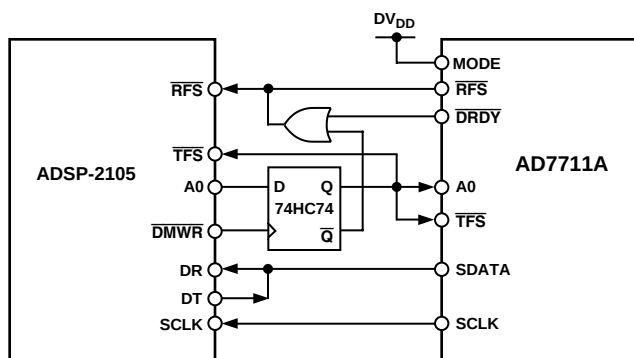
Figure 19. AD7711A to ADSP-2105 Interface
