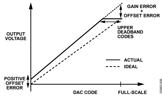
Figure 41. DAC Transfer Function with Positive Offset ( V_{\text{REF}} = V_{\text{DD}} )
