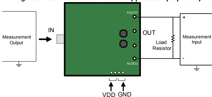
Figure 6—Connection for Audio Performance Test (Bottom View)
