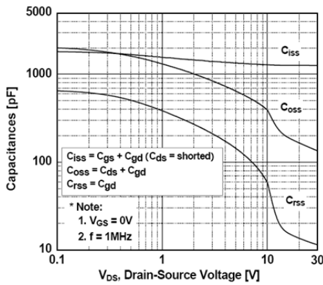
Fig. 5 Capacitance Characteristics
