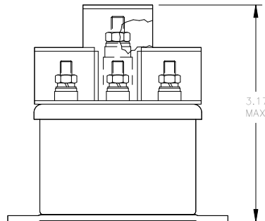
TERMINAL TYPE 7
