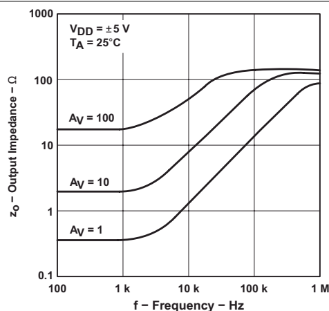
图 6-30. Output Impedance vs Frequency
