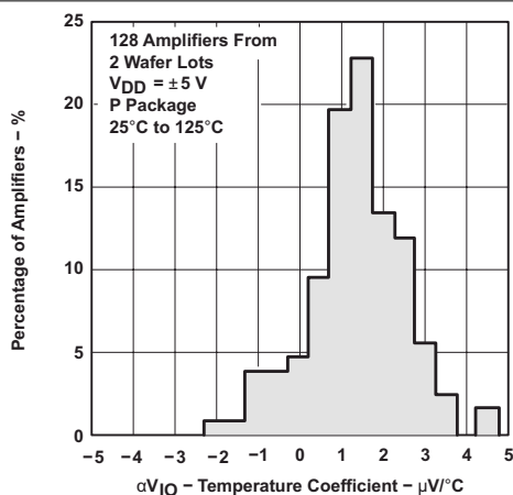
图 6-8. Distribution of TLC2272A-Q1 vs Input Offset Voltage Temperature Coefficient
