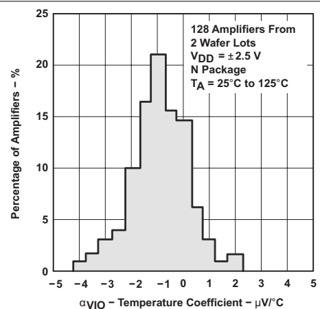
图 6-10. Distribution of TLC2274A-Q1 vs Input Offset Voltage Temperature Coefficient
