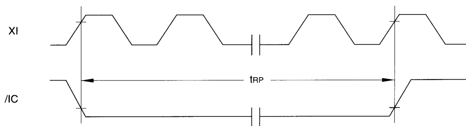
Fig. 2 Reset Timing
