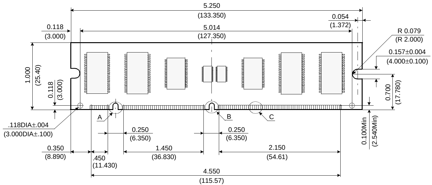
( Front view )
