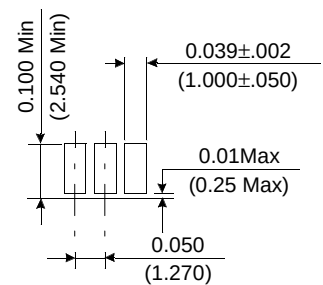
Detail C
