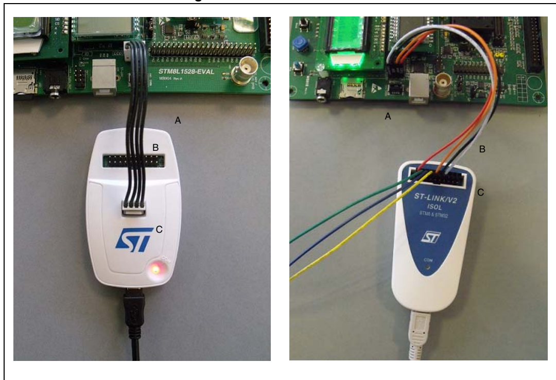
Figure 7. Low-cost connection
