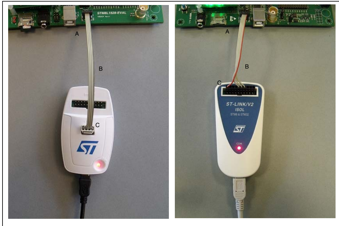
Figure 5. ERNI connection
