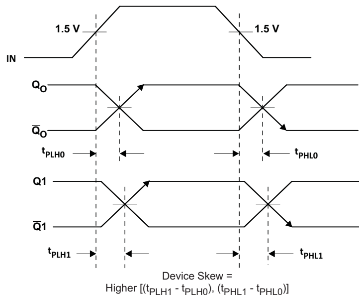
Figure 4. Device Skew
