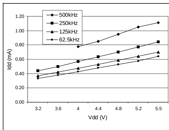
Figure 63. Typical I_{DD} in SLOW vs. f_{CPU}
