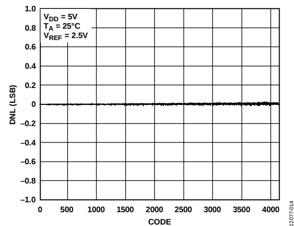
Figure 14. AD5691R DNL
