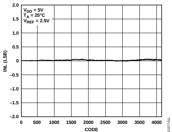
Figure 11. AD5691R INL
