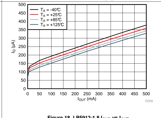
Figure 18. LP5912-1.8 I_{GND} vs I_{OUT}
