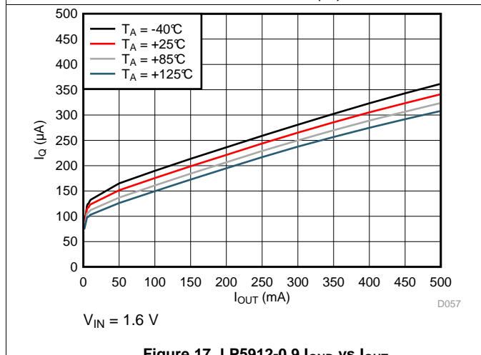
Figure 17. LP5912-0.9 I_{GND} vs I_{OUT}
