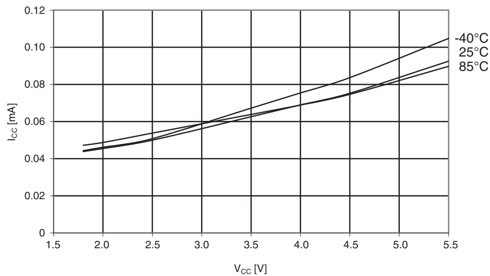
Figure 30-206. ATmega644A: Idle supply current vs. V_{CC} (internal RC oscillator, 128kHz)
