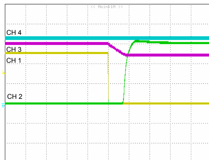
Figure 4: Oring for one feed loss (500µS/div):
